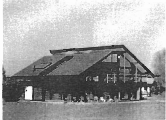
Hardacre Farm 2007: a German modular "Huf House" with laminated timber frame
