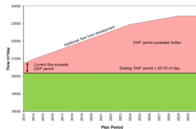
Figure E2.5 Canterbury - Headroom capacity phasing
