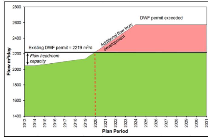
Figure E13.6: Paddock Wood - Headroom capacity phasing
