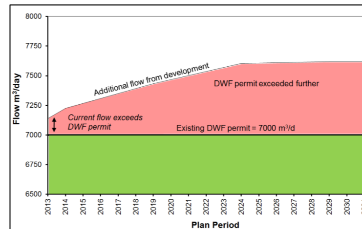
Figure E10.5: Faversham - Headroom capacity phasing
