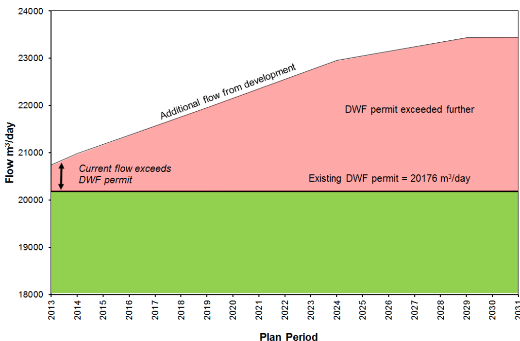
Figure C3: Canterbury WwTW DWF across plan period and DWF permit exceedance
